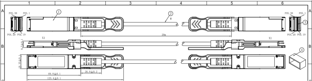
Mechanical Specifications
